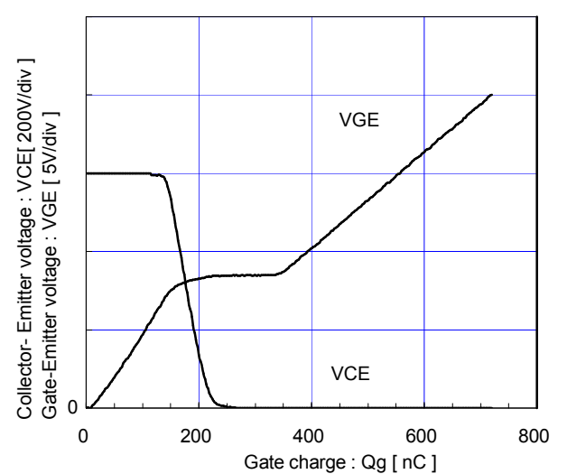
Dynamic Gate charge (typ.) Vcc=600V, Ic=150A, Tj=25°C
