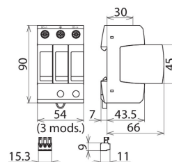
Dimension drawing DG M YPV 1500 FM
