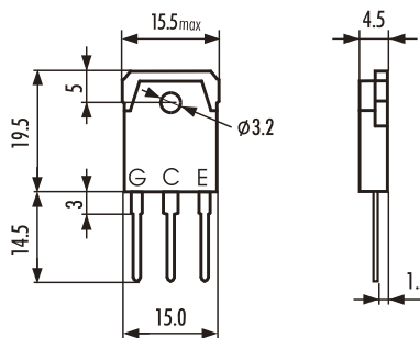
39 TO-3P
