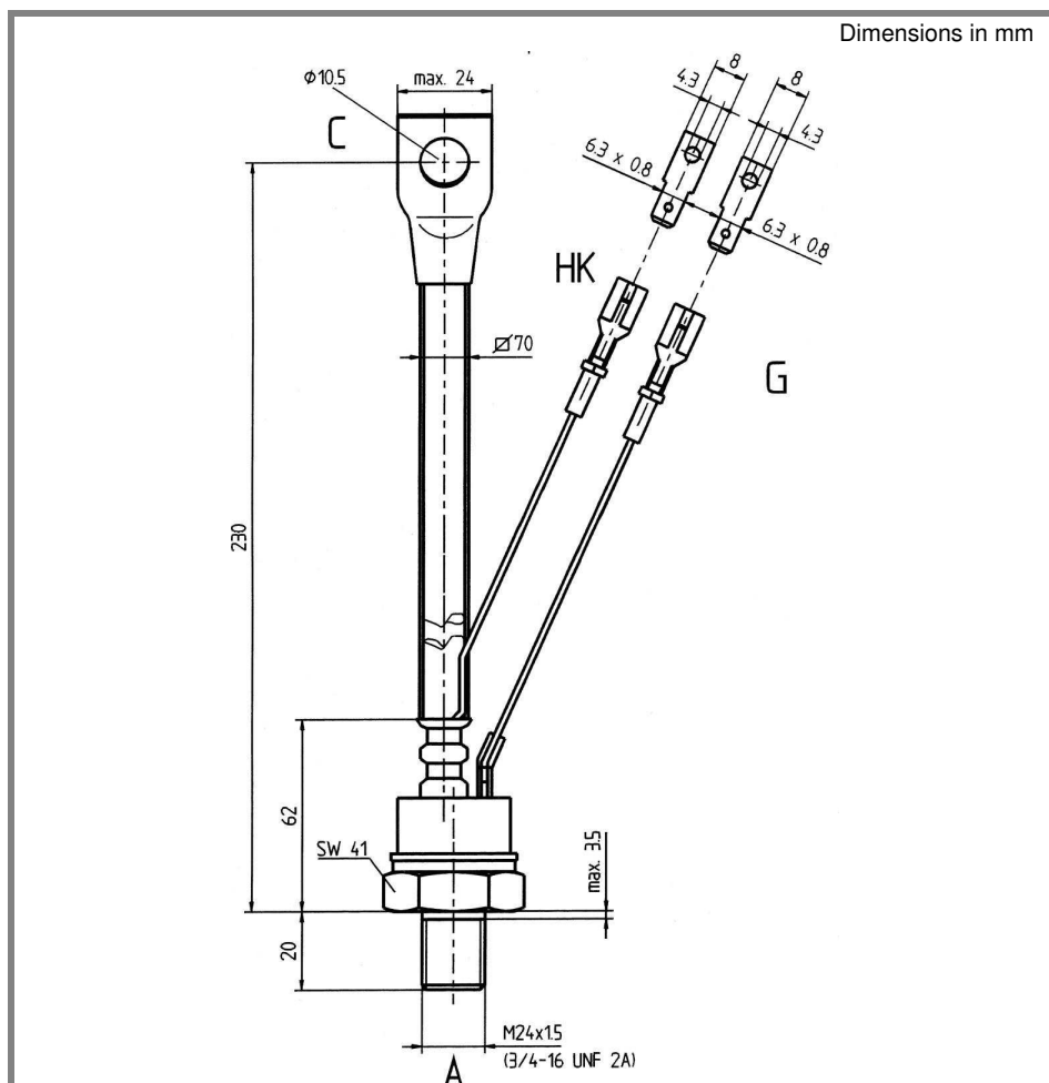
Case B 7 (IEC 60191-2: A29MA; JEDEC: TO-209AD (TO-118))
